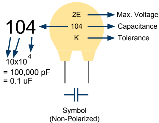
Ceramic Capacitor
