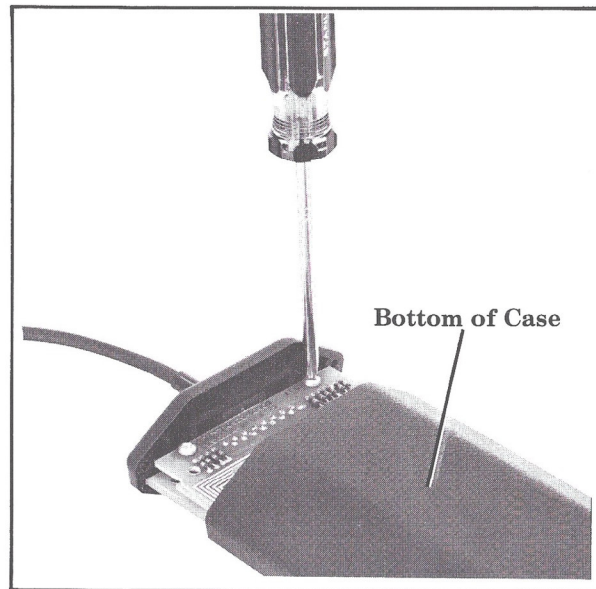
Figure 5-2. Removing Circuit Board Screws
