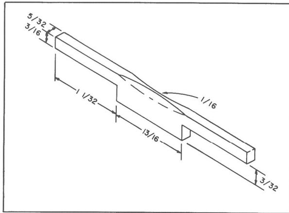
Figure 5-6. Extractor Tool
