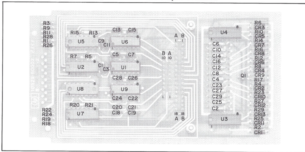
Figure 8-3. Main Board Component Locations
