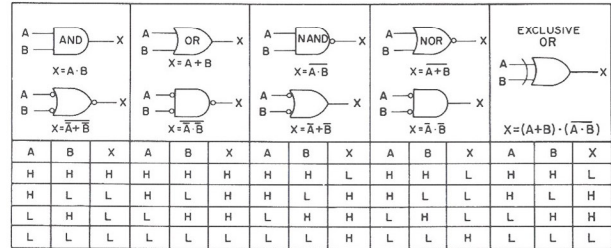
Figure 4-1. Gate Symbols and Logic Comparisons
