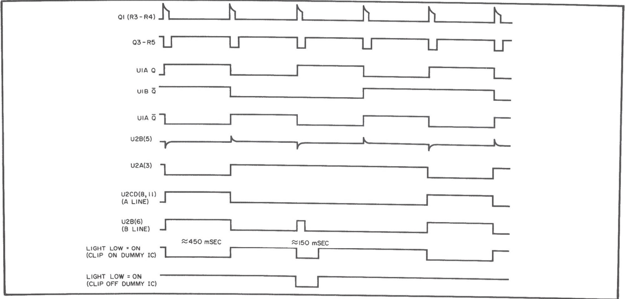
Figure 4-3. Test Card Timing Diagram
