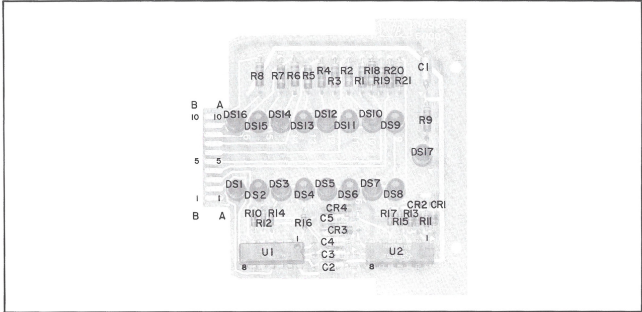
Figure 8-4. Display Board Component Locations
