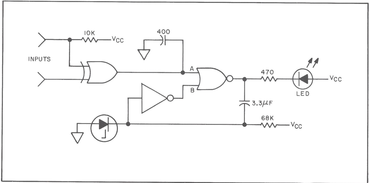
Figure 4-2. One Comparator Logic Channel Schematic
