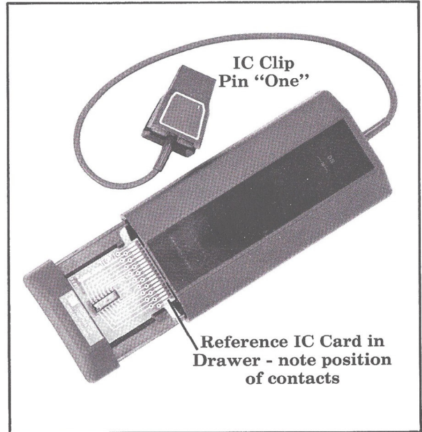
Figure 3-3. Reference IC Card in Comparator Drawer
