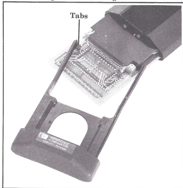
Figure 5-3. Removing Drawer
